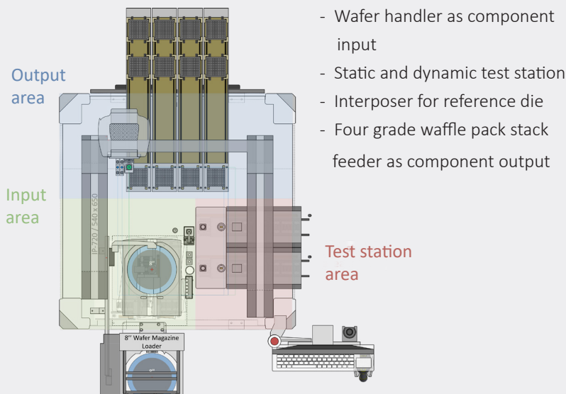
KGD Test Handler 8" Wafer
