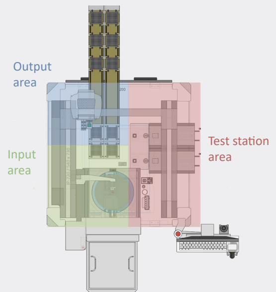
KGD Test Handler 12" Wafer
